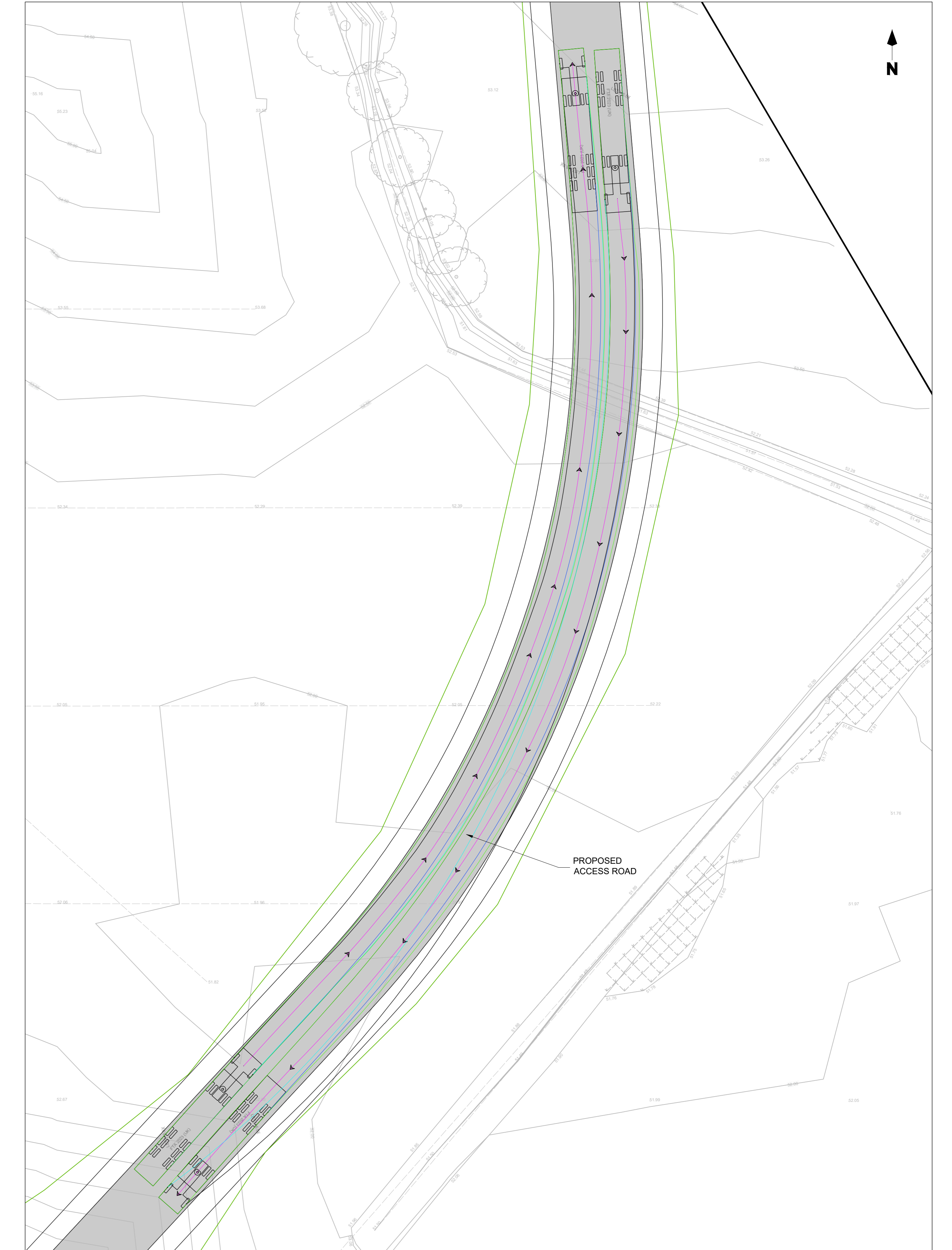
100m BEND TRACKING Scale 1:250
